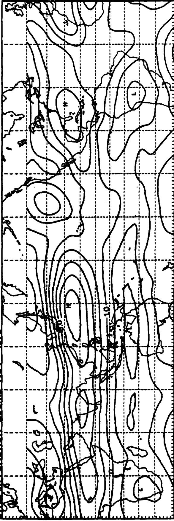
STREAM FUNCTION 200MB NOV 1978
